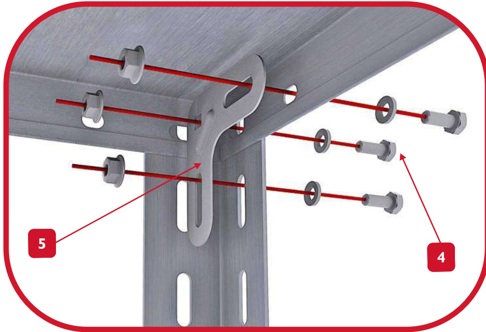
Detail of square, shelve and anglebolted system
